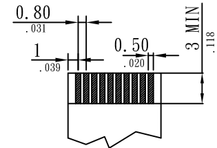
FFC/FFC DIMENSION THICKNESS 0.3mm
