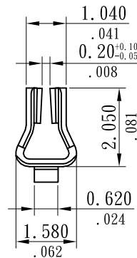
C-C SECTION
