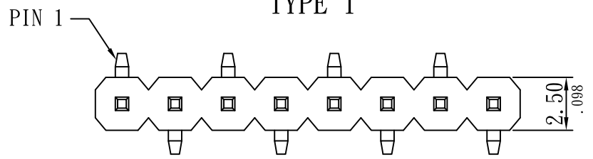
PCB LAYOUT TYPE 1
