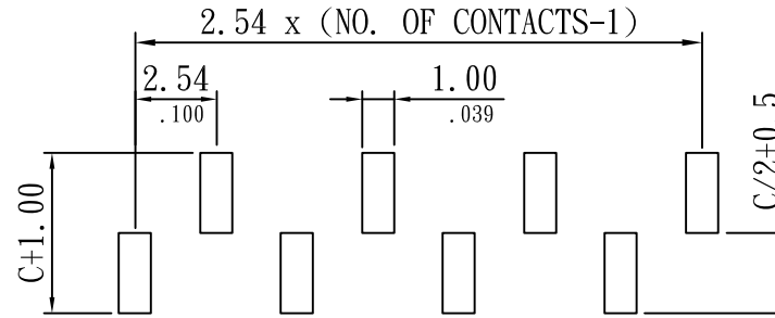
PCB LAYOUT TYPE 2
