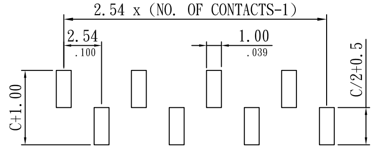
PCB LAYOUT TYPE 1
