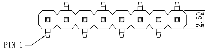
PCB LAYOUT TYPE 2
